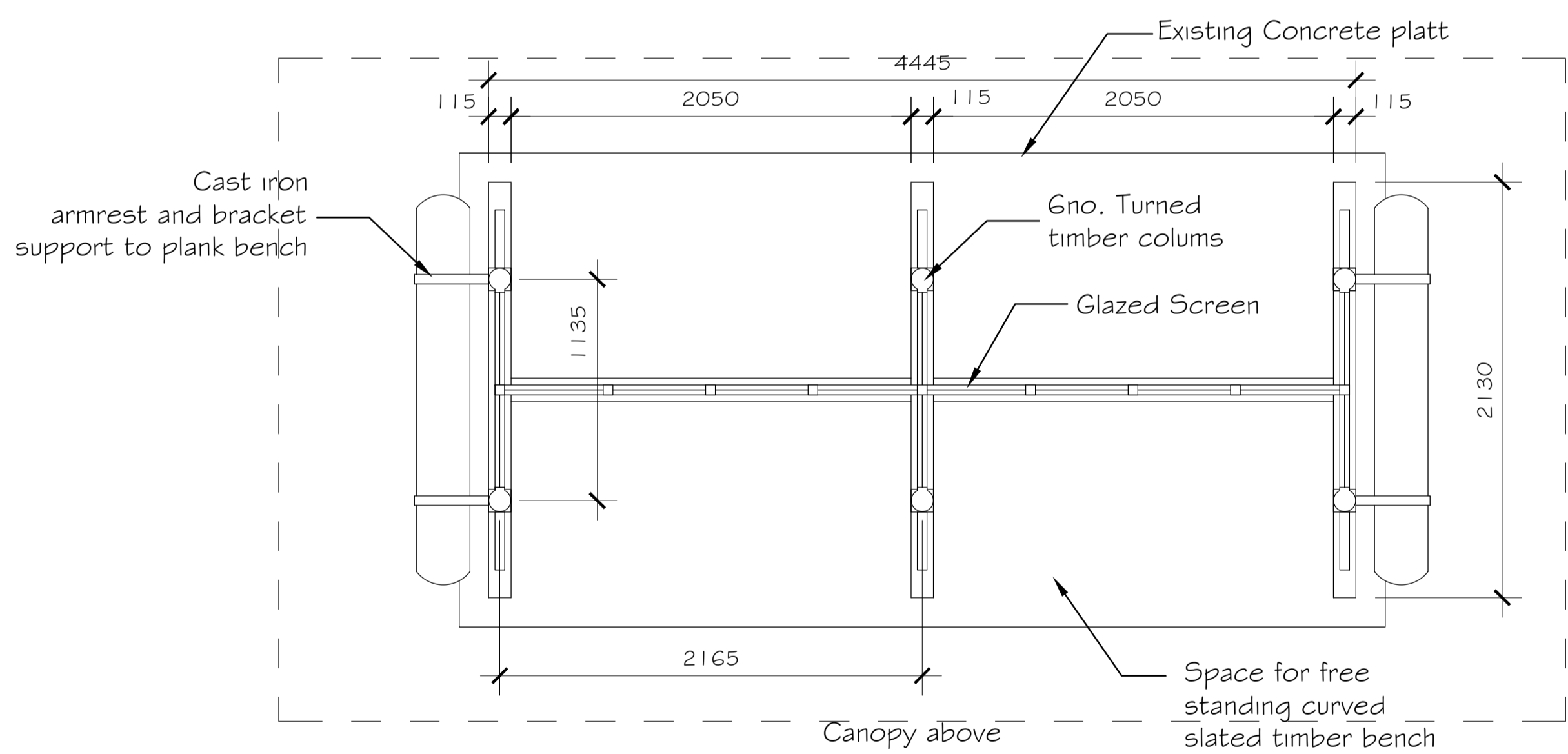
Existing Plan (All sizes to be checked on site)
